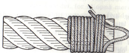
Fig. 8-213. Almindelig takling.
